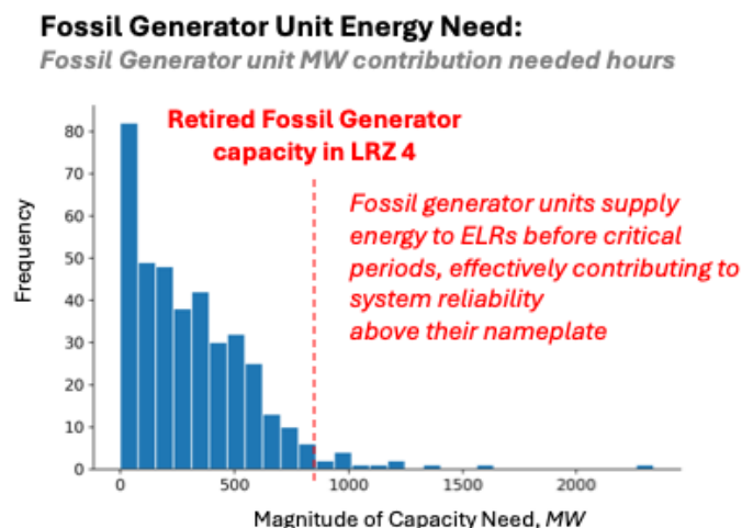
Figure 5-38: LRZ 4 Fossil Generators Contribution in Needed Hours
