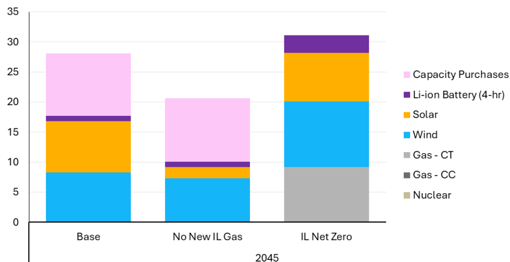
Figure 5-46: 2045 MISO LRZ 4 Selected Nameplate Capacity (GW)
